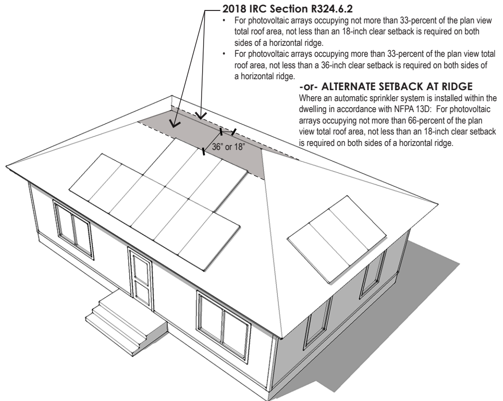
FIGURE 4: DWELLINGS AND HABITABLE DETACHED STRUCTURES WITH ROOF SLOPED MORE THAN 2:12
